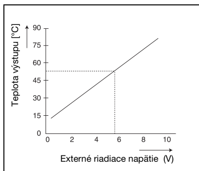
Obr. 3 0 – 10V Diagram
