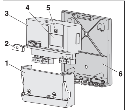
fig. 1 Overview EM10 pos. 1: Terminal cover pos. 2: Fuse holder pos. 3: Module EM10 pos. 4: Identification plate pos. 5: Operational/fault LED pos. 6: Wall bracket
